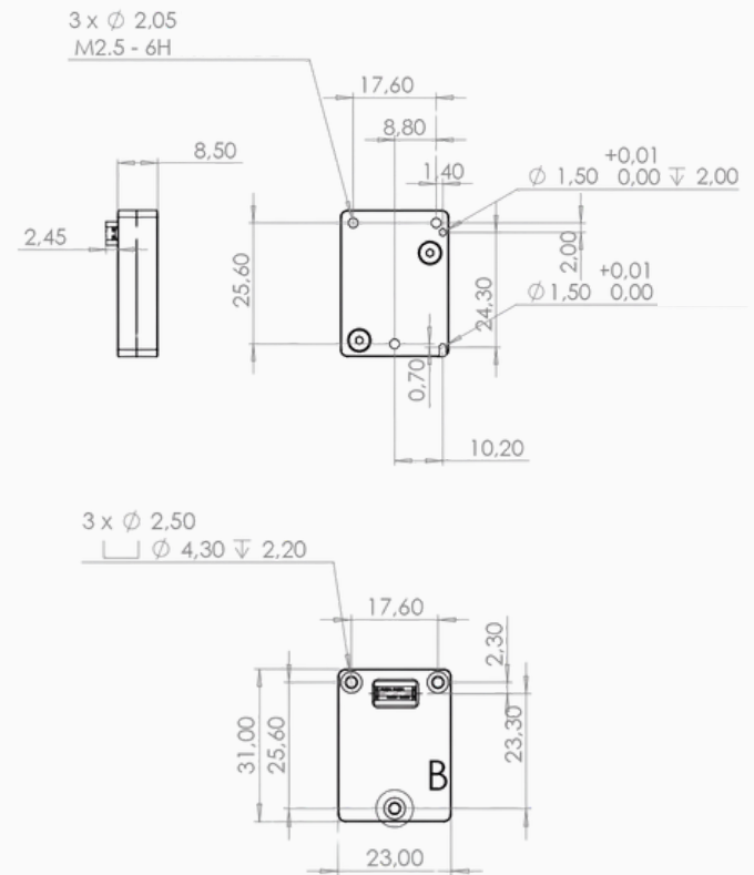
K-PUS Micro series mechanical drawing dimensions are in mm
